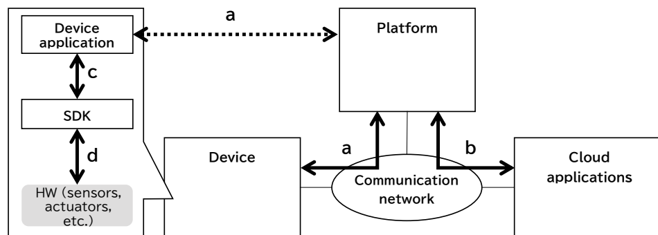
Figure 3-5 Interface list
