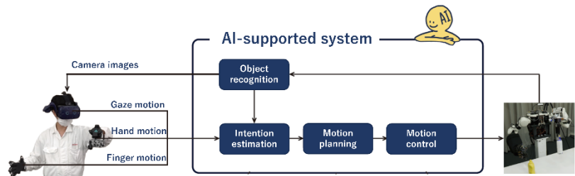
Figure 4-13 AI-supported remote control
