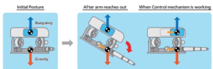
Figure 4-16 Mechanism to Control Center of Buoyancy and Center of Gravity
